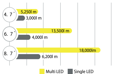
LUMEN OUTPUT COMPARISON
